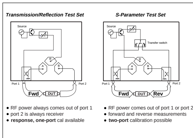
Figure 9. T/R versus S-Parameter Test Sets
