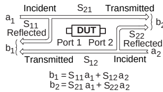
Figure 16. Limitations of H, Y, and Z Parameters (Why Use S-parameters?)
