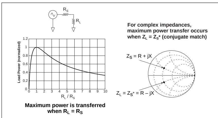
Figure 7. Power Transfer
