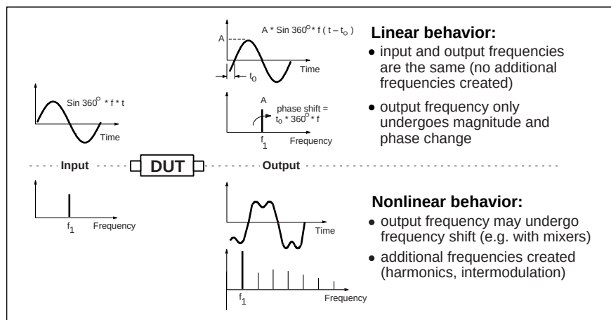
Figure 1. Linear versus Nonlinear Behavior
