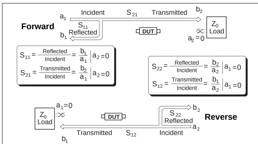
Figure 17. Measuring S-Parameters
