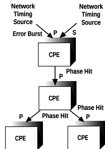
Figure 15. Cascading errors in private networks.
