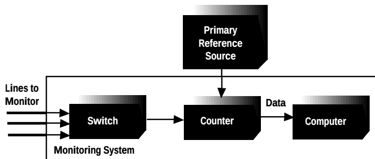
Figure 13. Synchronization Monitoring System.
