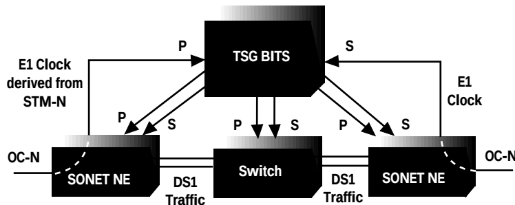
Figure 14. Timing distribution using SONET lines.
