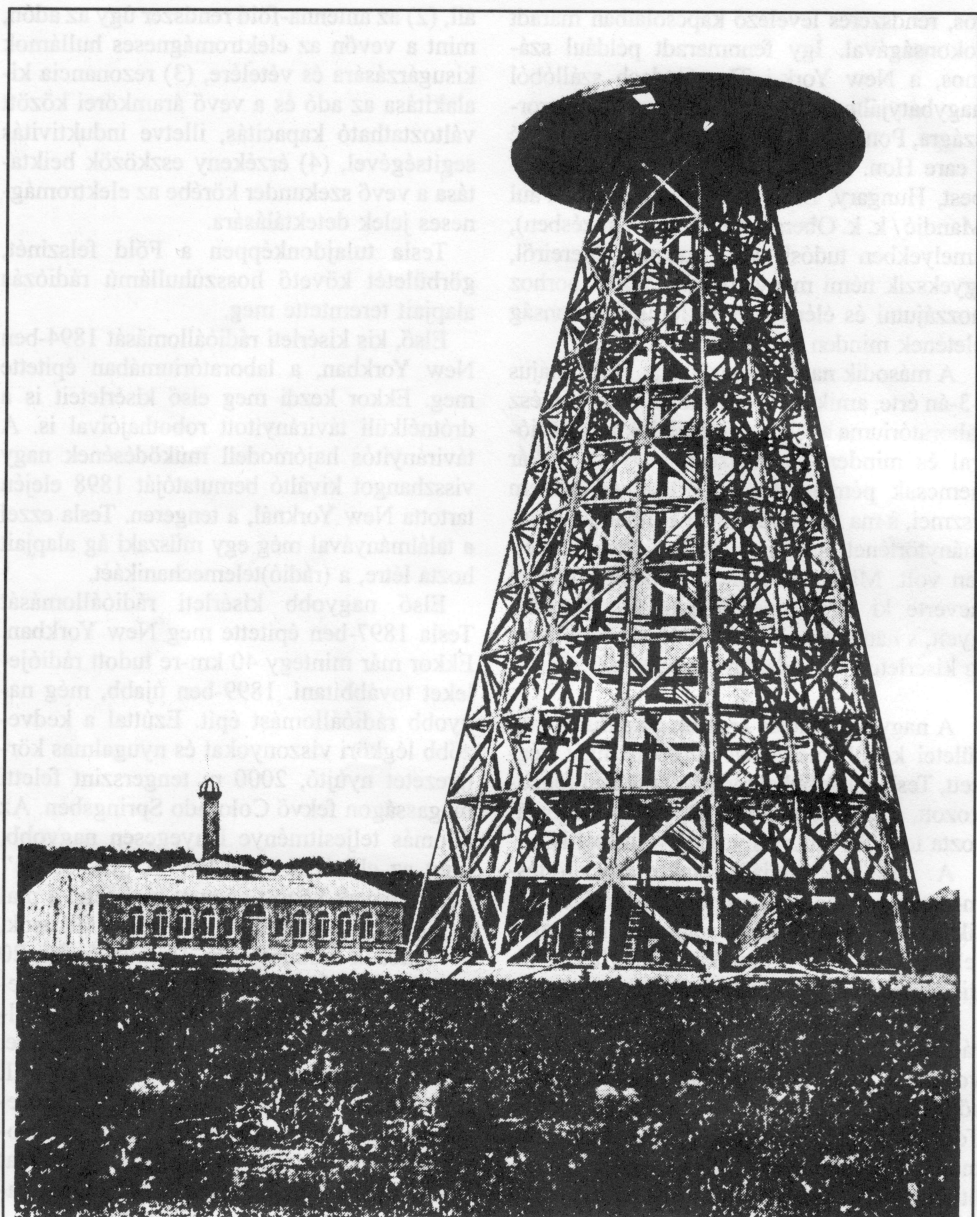
Central Power Plant, Transmitting Tower, and Laboratory for "World Telegraphy," Wardenclyffe, Long Island.
